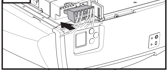
Fig. 44 Terminal block XB03
