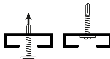
IMAGE 2: Attaching the ME110-C mounting channel
