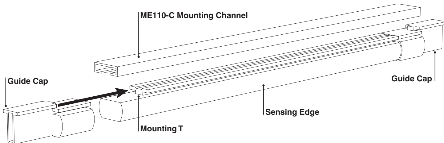
IMAGE 1: MC110 Sensing edge, guide cap, and mounting channel assembly
