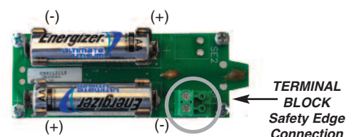
Fig. 2-6 WIRE CONNECTION TO TERMINAL BLOCK
